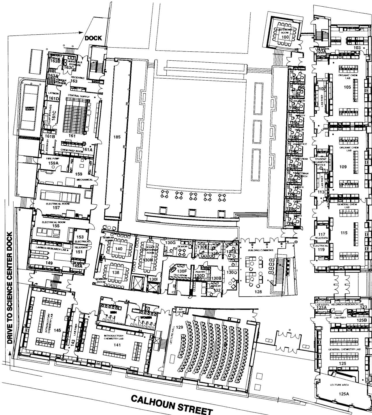
COLLEGE OF CHARLESTON NEW SCIENCE CENTER BUILDING CHARLESTON, SC FLOOR 1
